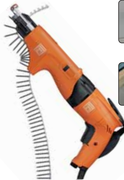
SCT 5-40 M
